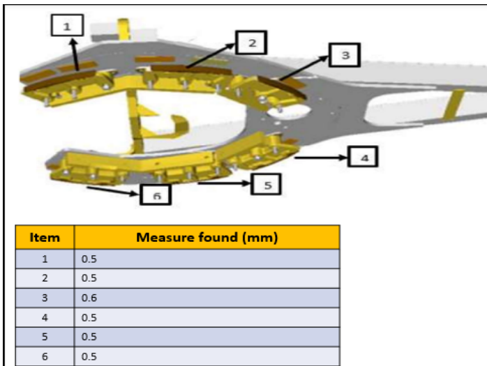
Image 4 - Identification and blank filling spaces table
