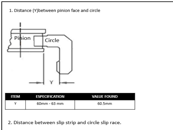
Images 2 and 3 - Procedure instructions containing parts identification, specification measurements and a blank space to fill with the found measure
